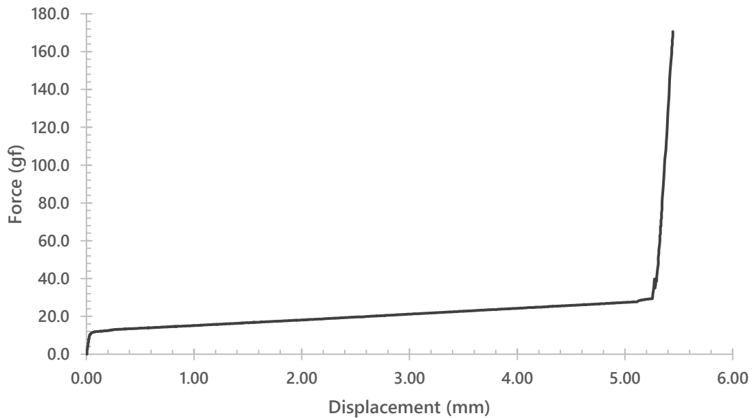
Niz EC Linear UHMWPE 15g (Upstroke)
